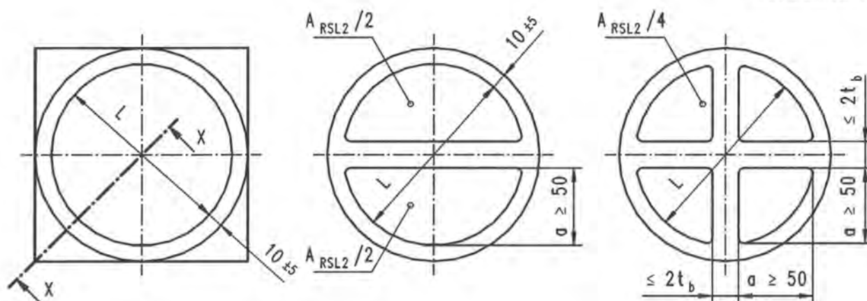
Figure H.2 - Examples of recessed flat ROBO®SLIDE L2 configurations
