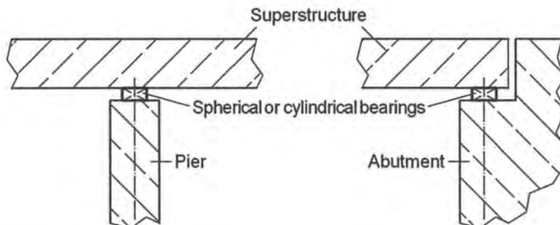
Figure A.1 - Assembly of a guided and free movable mageba RESTON®Spherical and Cylindrical Bearings and its intended use (example)
