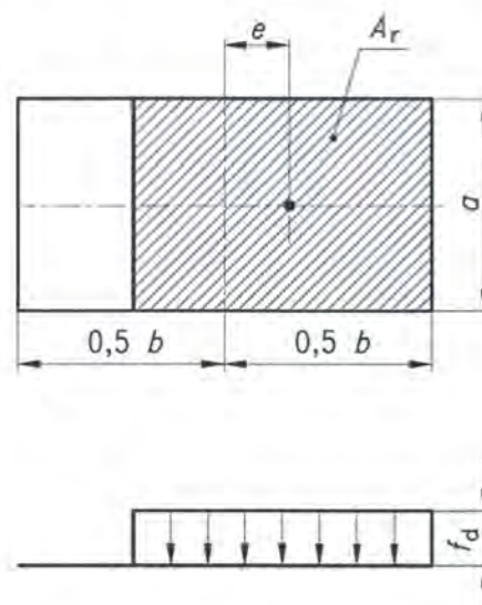
Figure I.2 - Reduced contact area A_r for rectangular sliding surfaces.
