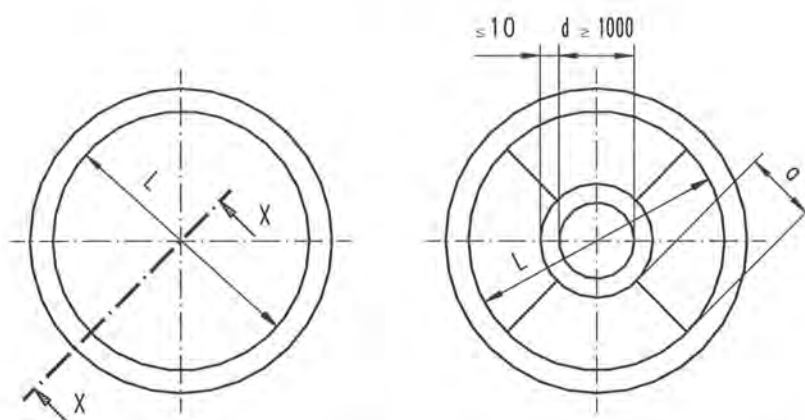
Figure H.3 - Subdivision of recessed ROBO®SLIDE L2 sheets for spherical sliding surfaces
