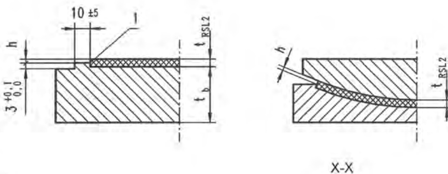
Figure H.1 - Details of ROBO®SLIDE L2 recess and relief
