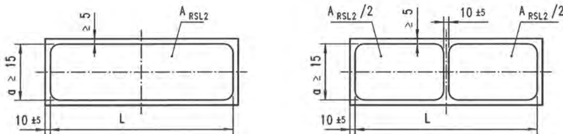
Figure H.4 - Examples of recessed ROBO®SLIDE L2 sheets for guides
